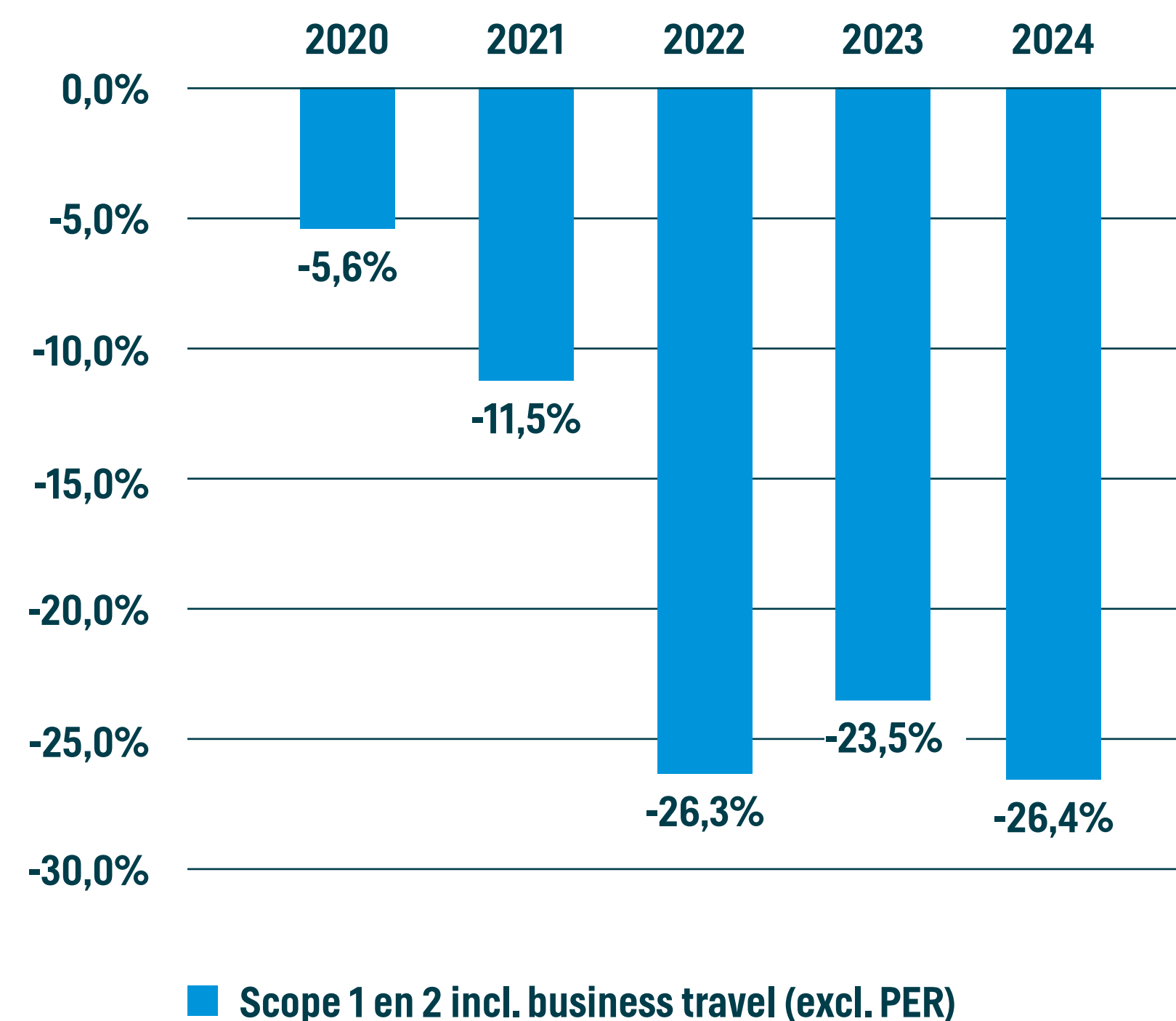
Trend CO 2 emissie Scope 1 & 2 versus 2019
